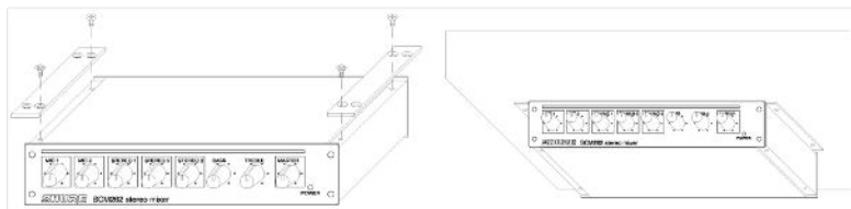
Hanging Mount
